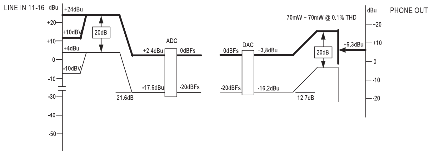
LEVEL DIAGRAM
